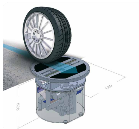
Image 2: Via laser diode-digital cameras, which are fit into shafts in the highway or troughs, tire treads depths can be captured and calculated in milliseconds by the integrated DIN rail PC, Kontron ThinkIO.
